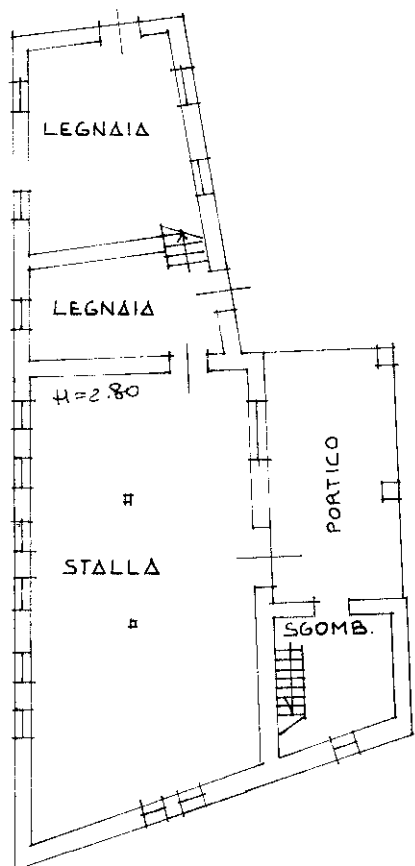
PIANO TERRA
