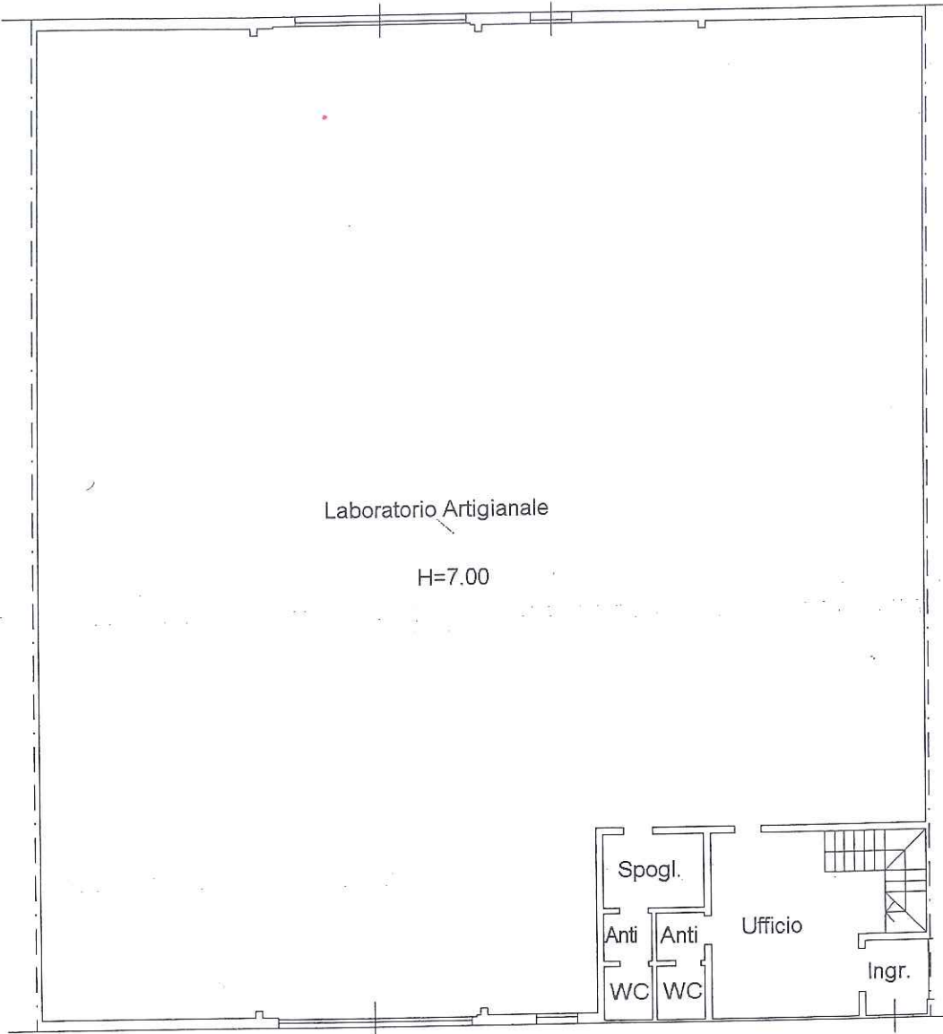
PIANTA PIANO TERRA p T H=2.70
